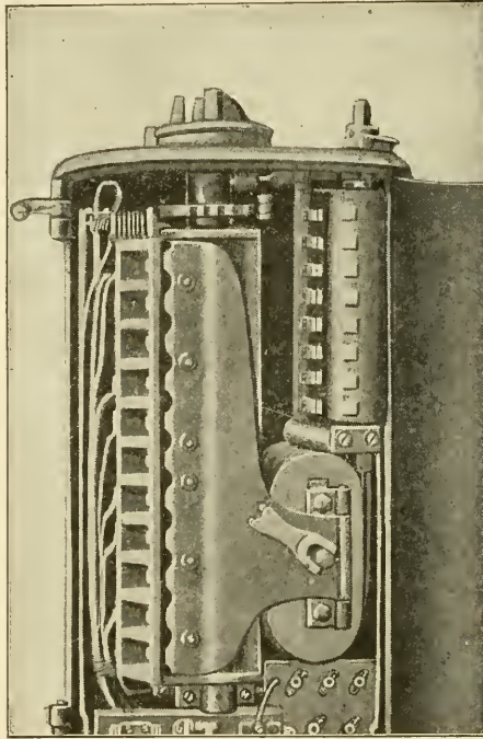
Fig. 77. Current Limit Relay Used by Denver Railway Company
